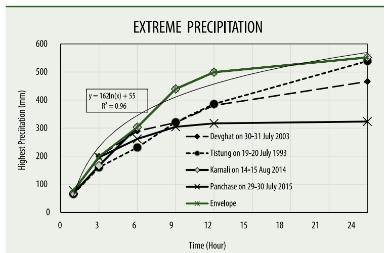
Figure 4: Comparison of Three Severe Precipitation Events Maximized for Different Durations
